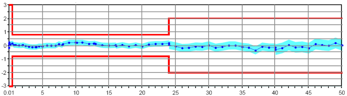
Diagram: Output power accuracy in dB versus frequency in GHz of the R&S®ZVA50.
