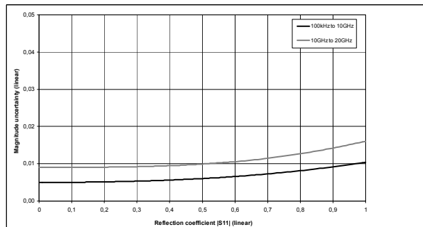
Typical accuracy of reflection magnitude and reflection phase measurements for the R&S ® ZNB20 in the frequency range from 100 kHz to 20 GHz. Analysis conditions: S_{12} = S_{21} = 0 , cal. power –10 dBm, meas. power –10 dBm.
