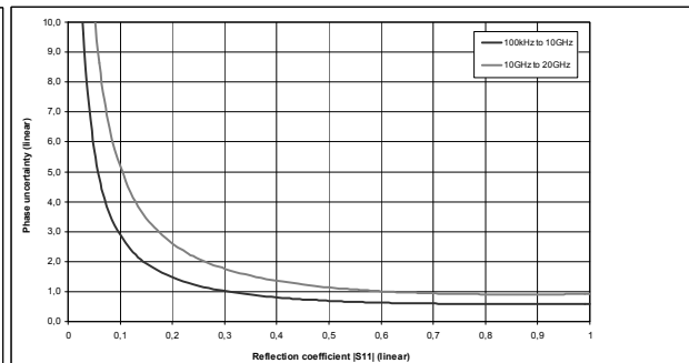
Typical accuracy of reflection magnitude and reflection phase measurements for the R&S ® ZNB20 in the frequency range from 100 kHz to 20 GHz. Analysis conditions: S_{12} = S_{21} = 0 , cal. power –10 dBm, meas. power –10 dBm.
