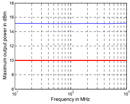
Maximum output power in dBm versus frequency for the R&S® ZNB40.
