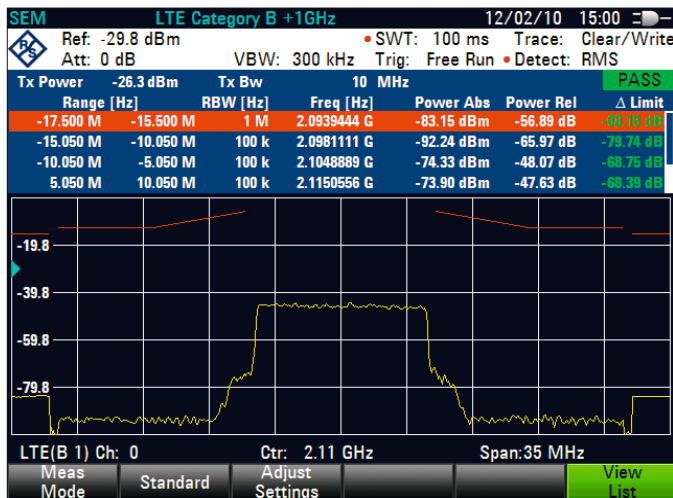
Spectrum emission mask measurement on an LTE signal.
