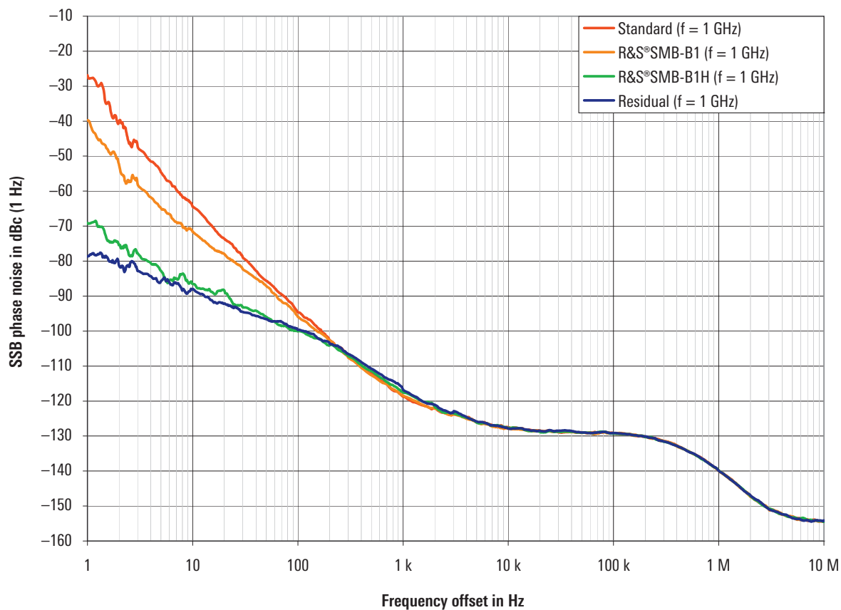
SSB phase noise comparison with standard internal reference, R&S ® SMB-B1, R&S ® SMB-B1H (meas.) and residual phase noise.
